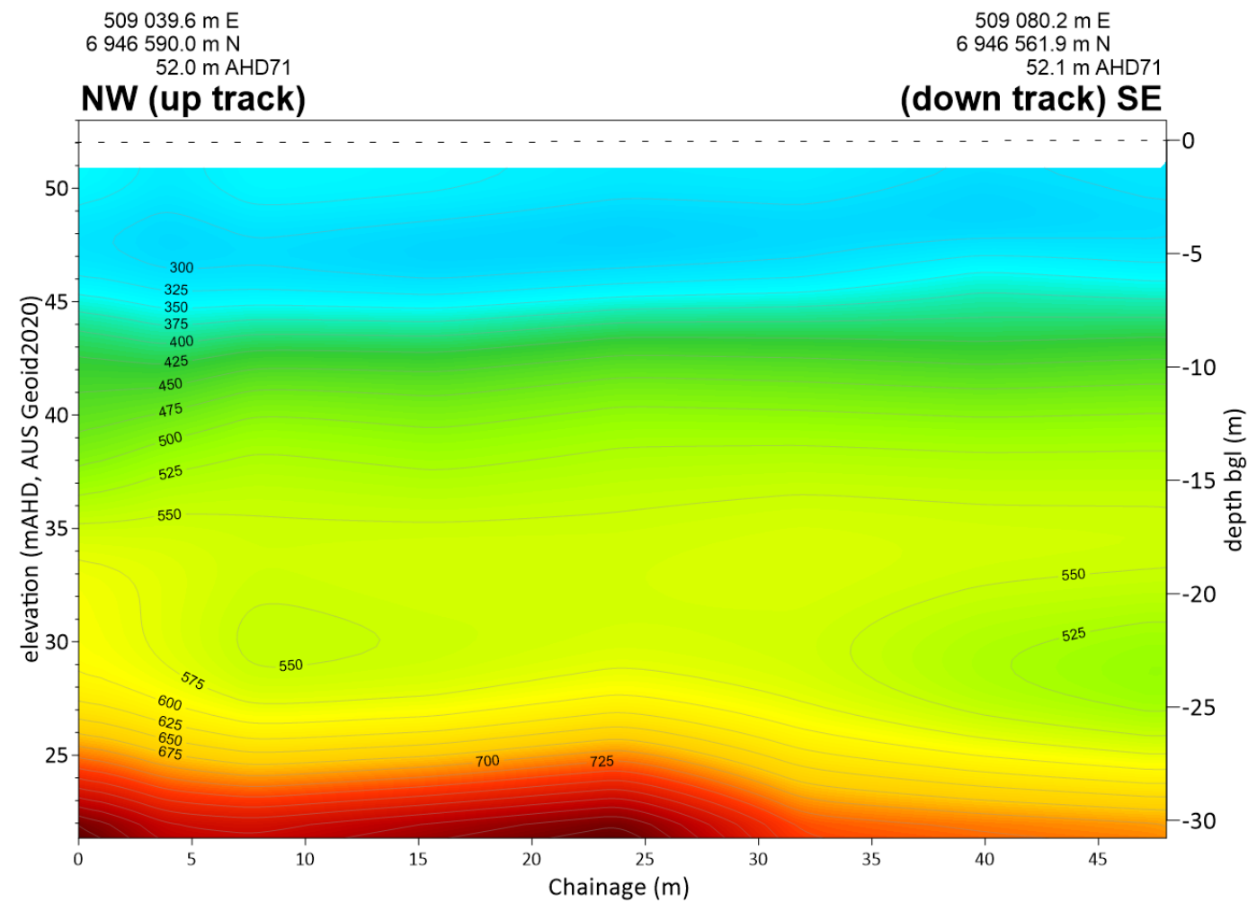
Seismic Line MASW AU-GP 103
